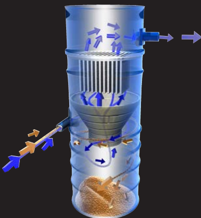
Cleaning of production machinery. Vacuum extraction of flour and bread particles.
