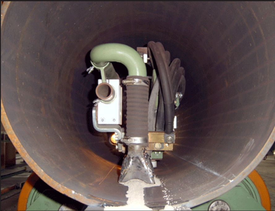
Extraction of welding powder during longitudinal seam welding
